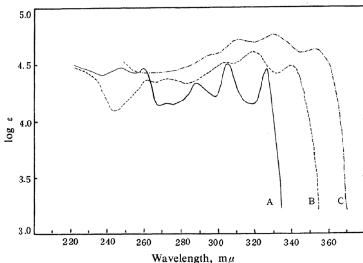
Fig. 3. Ultraviolet absorption spectra.
