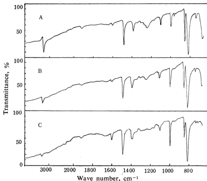
Fig. 1. Infrared absorption spectra.
