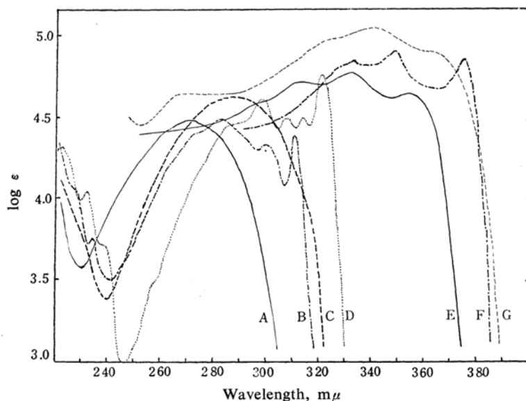
Fig. 2. Ultraviolet absorption spectra.
